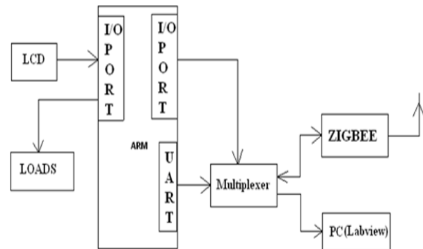
Fig.2. Block diagram of computer side
