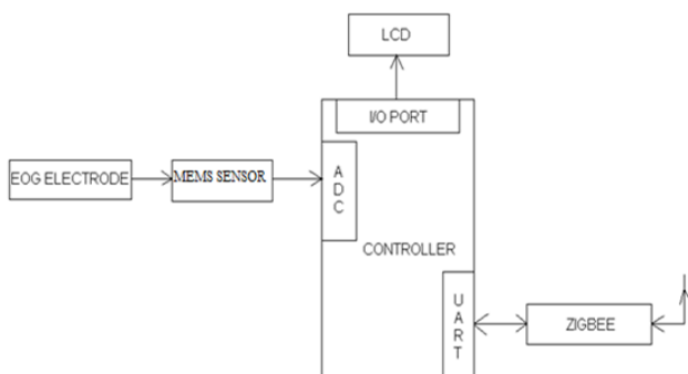
Fig.1. Block diagram of Human side
